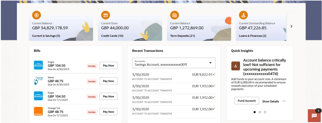
Figure 1-1 Overview widget
